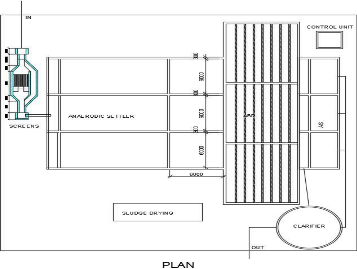
Fig. 2: Layout Plan
