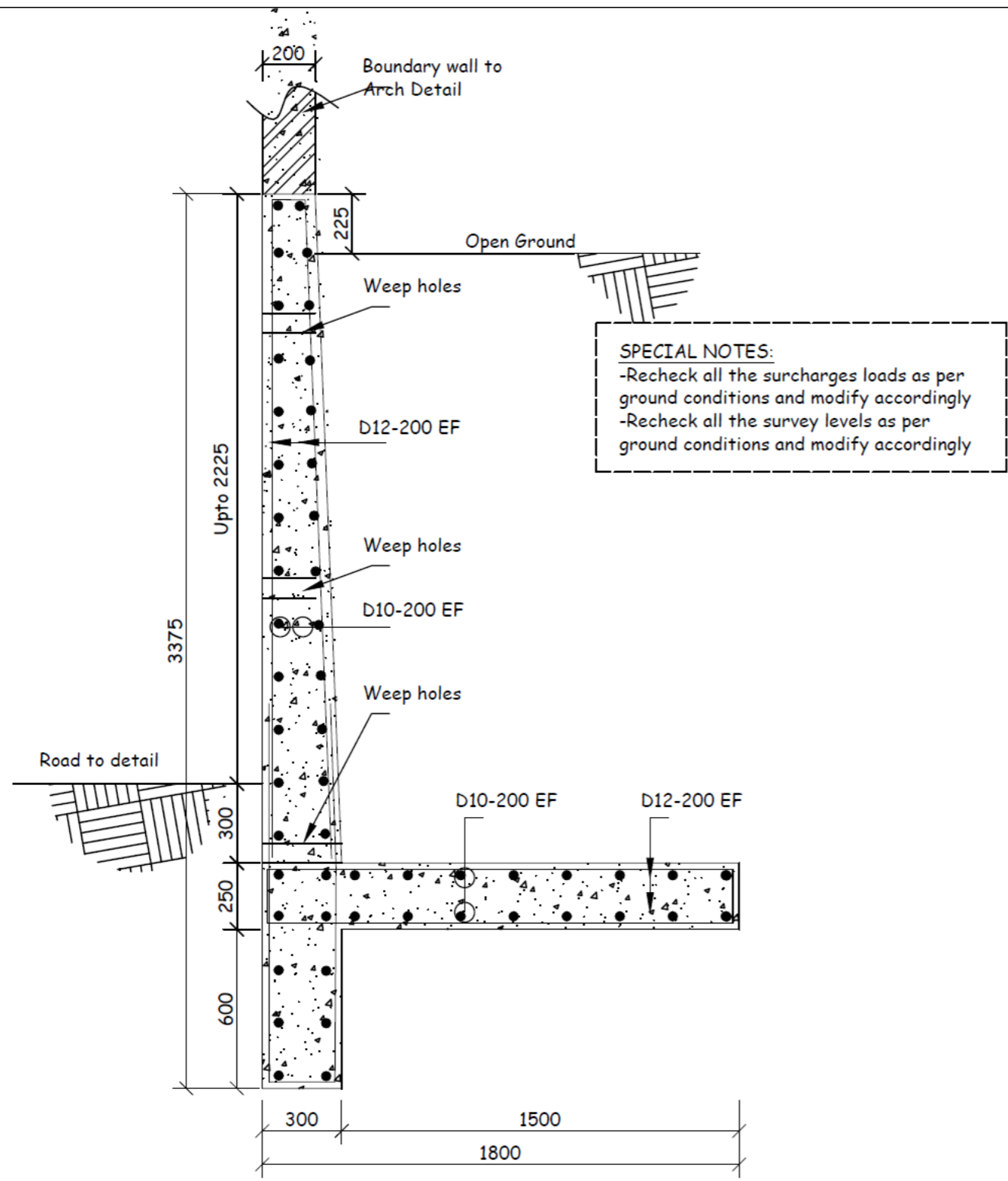
RETAINING WALL SECTIONAL R.C. DETAILS
