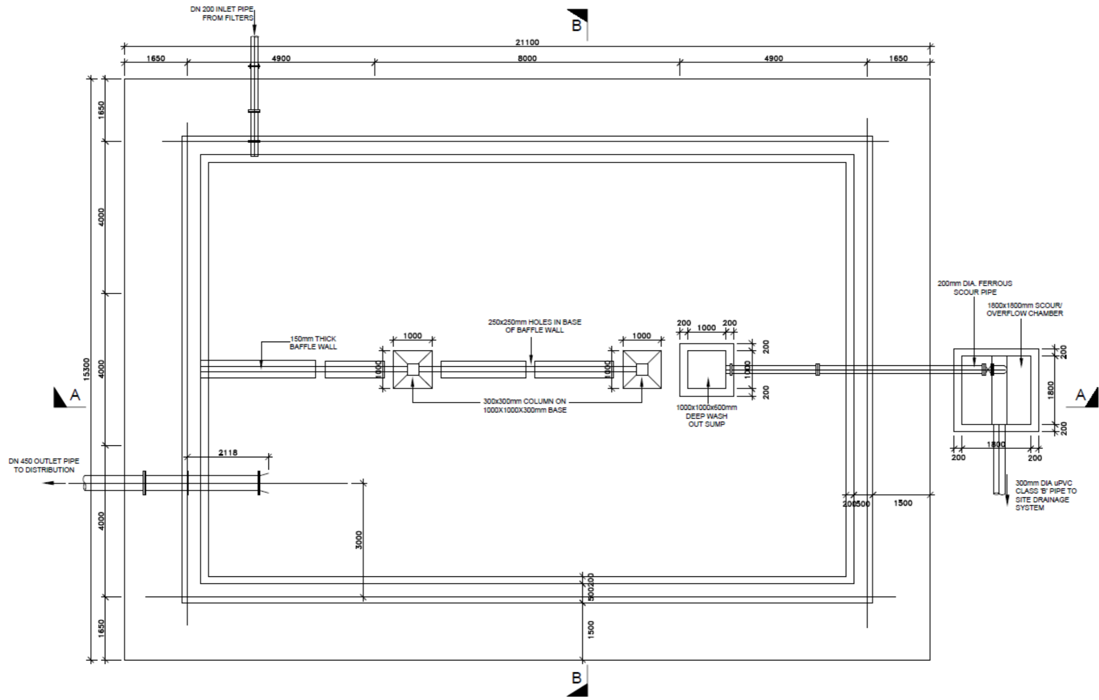
TREATED WATER TANK (500m 3 ) BASE SLAB PLAN
