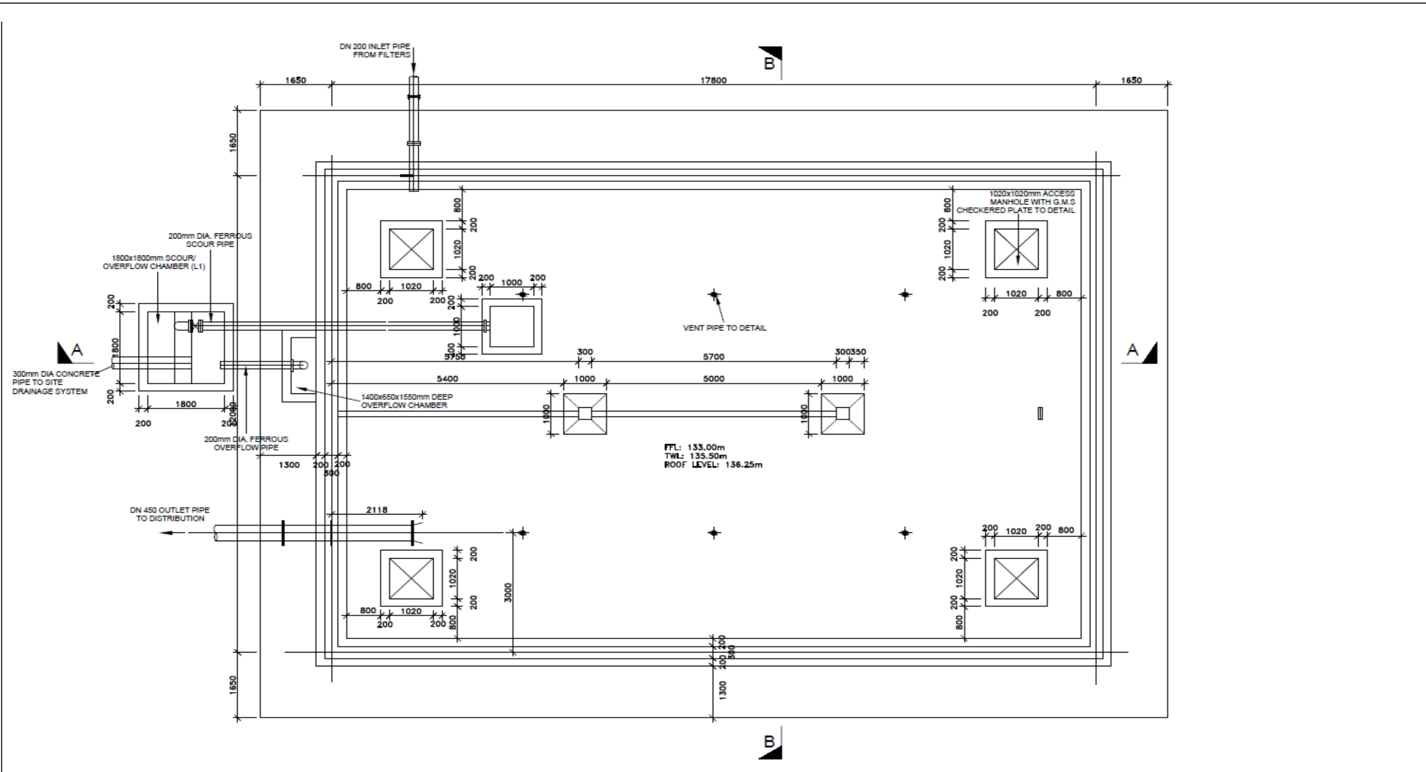
TREATED WATER TANK (500m 3 ) ROOF PLAN
